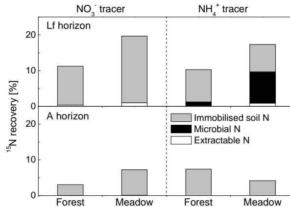
Figure 6. Total 15 N recovery of added NO 3 - and NH 4 + tracers in the soil pool fractions: immobilised soil N, microbial N, and extractable N in LF and A horizons in the experimental forest and meadow catchment in 2001 and in 2003. Extractable N is mainly DON with a negligible amount of extractable NO 3 - and NH 4 + .
