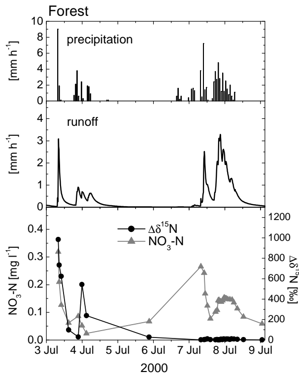
Figure 2. Runoff from the experimental forest catchment, its concentration in NO 3 - and \Delta\delta^{15}\text{N} during two rainfall events in July 2000.
